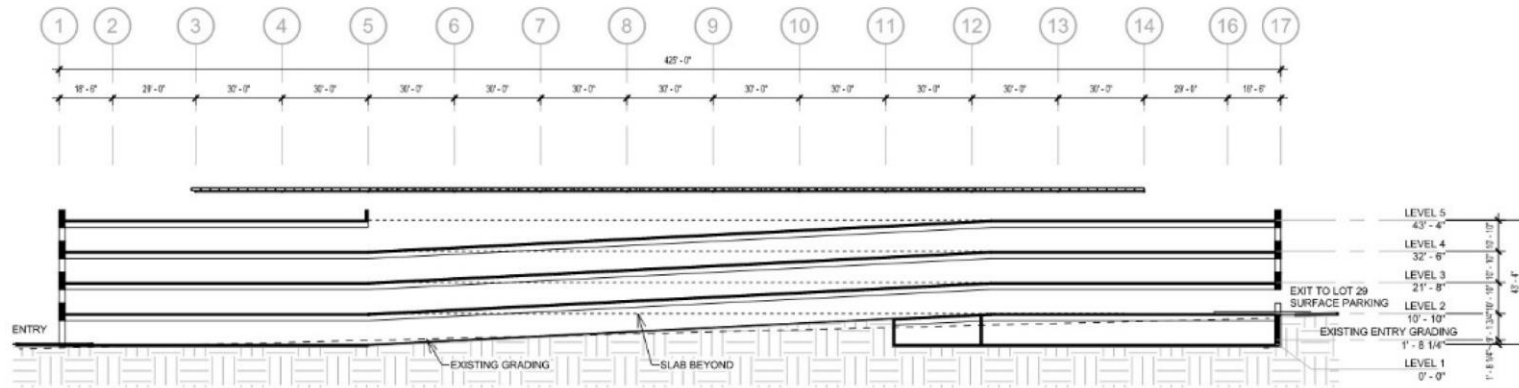
EAST-WEST BUILDING SECTION - OPTION 1
