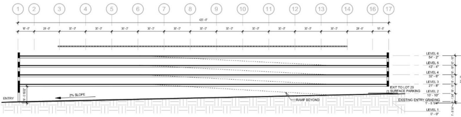
EAST-WEST BUILDING SECTION - OPTION 2
